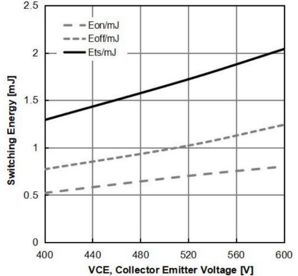
Figure 16: Typical Switching Energy vs. VCE ( T_J=25^\circ\text{C}, V_{GE}=15/0\text{V}, I_C=30\text{A} )
