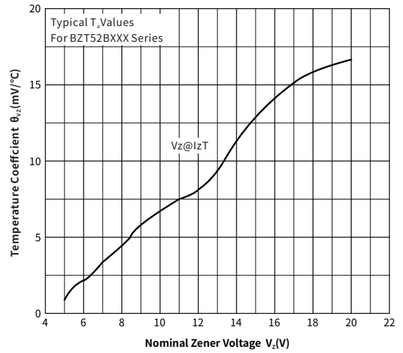
Fig. 2 Temperature Coefficients
