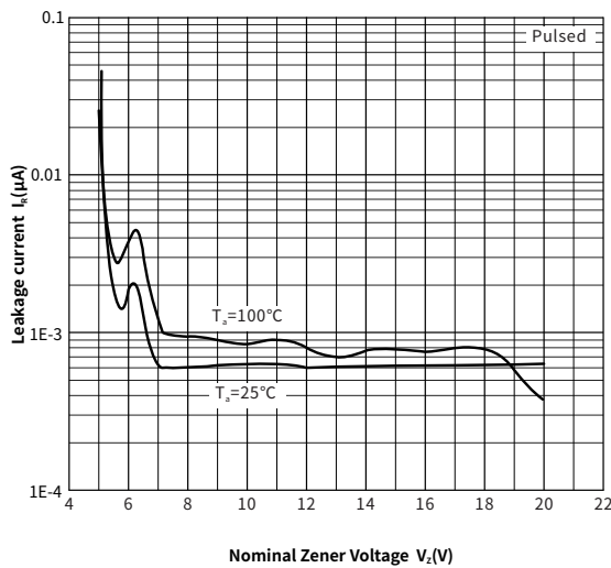
Fig. 3 Typical Leakage Current
