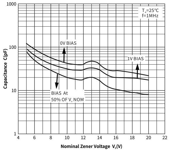
Fig. 4 Typical Capacitance
